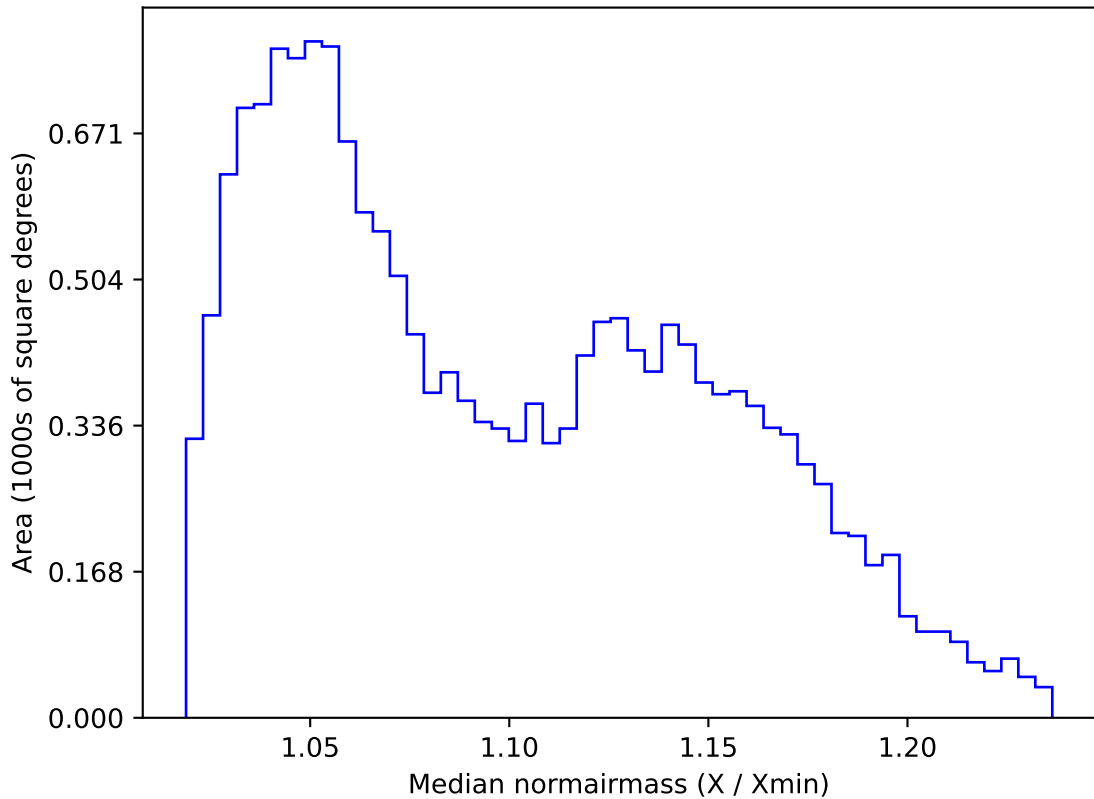
weather_cloudso10v3.4_10yrs WFD g band: Median normairmass
