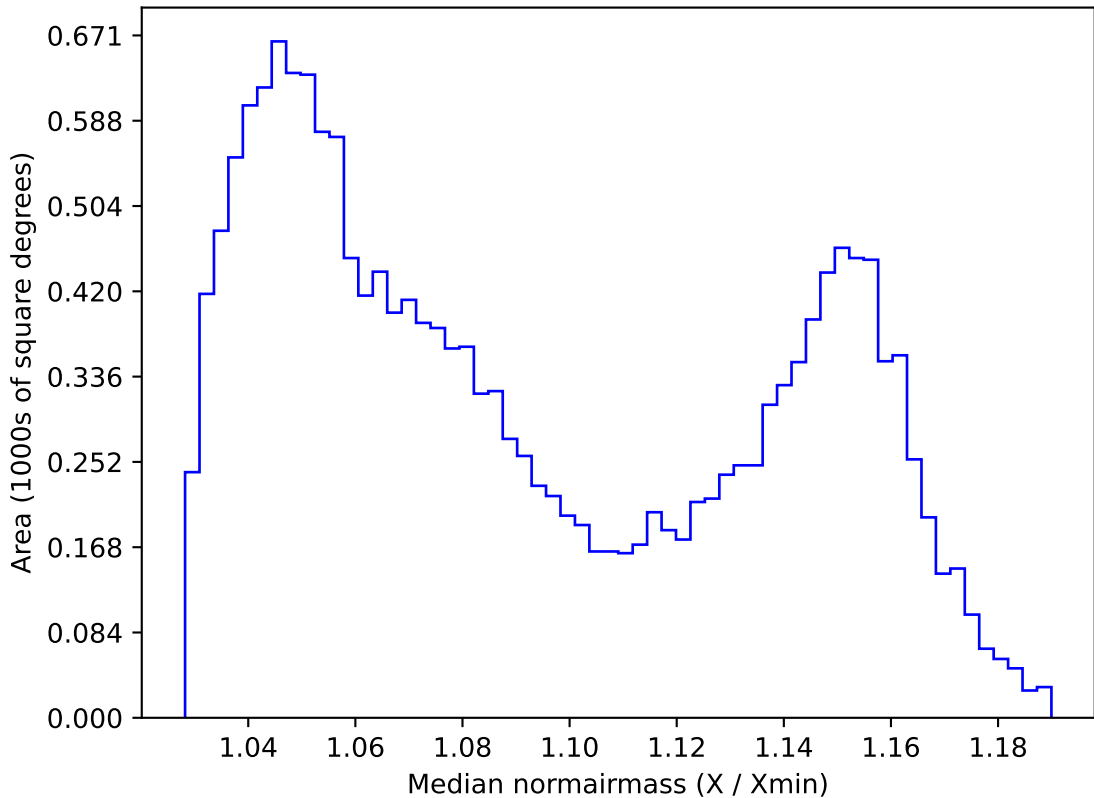
weather_cloudso10v3.4_10yrs WFD all bands: Median normairmass
