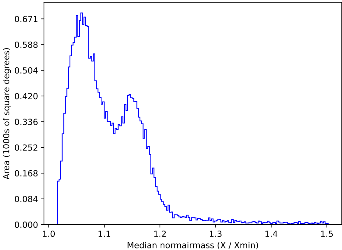
weather_cloudso10v3.4_10yrs All sky z band: Median normairmass
