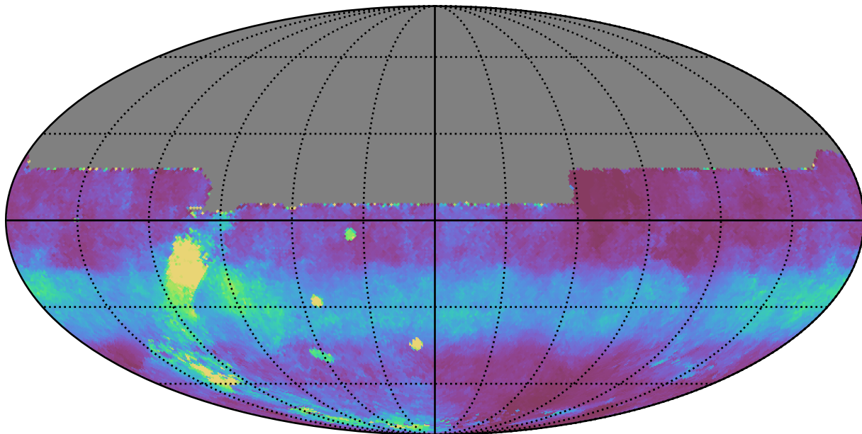
weather_cloudso10v3.4_10yrs All sky y band: Median normairmass
