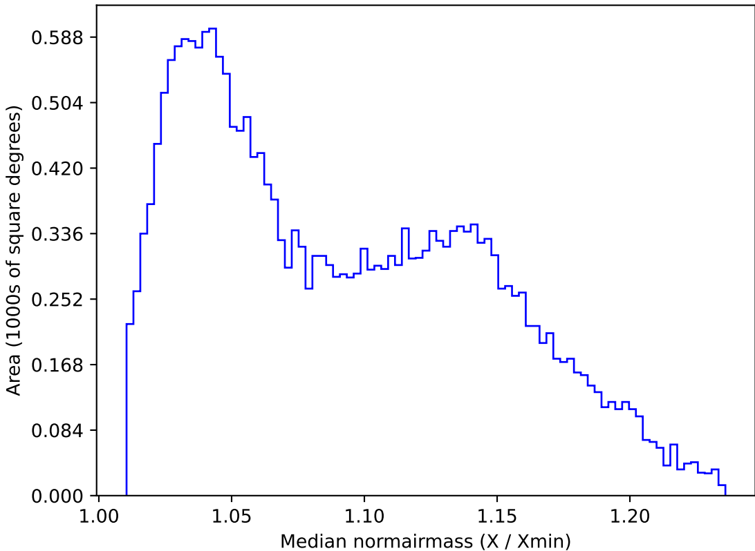
weather_cloudso10v3.4_10yrs All sky u band: Median normairmass
