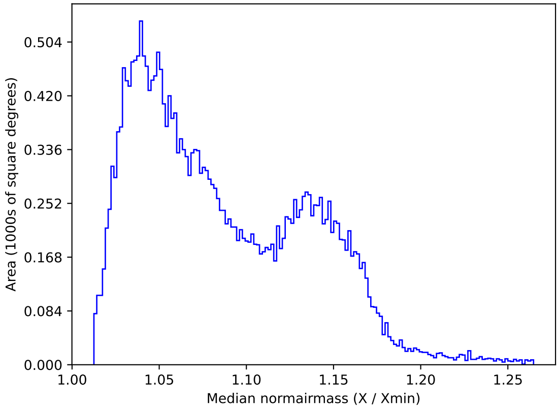
weather_cloudso10v3.4_10yrs All sky r band: Median normairmass
