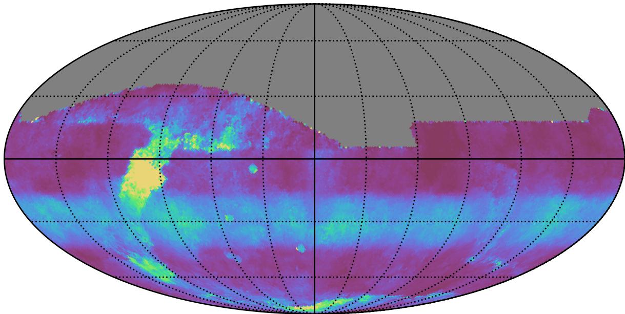
weather_cloudso10v3.4_10yrs All sky i band: Median normairmass
