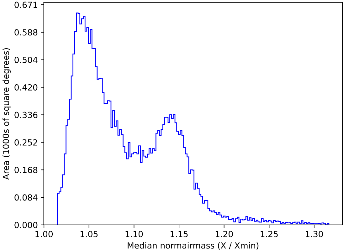
weather_cloudso10v3.4_10yrs All sky i band: Median normairmass
