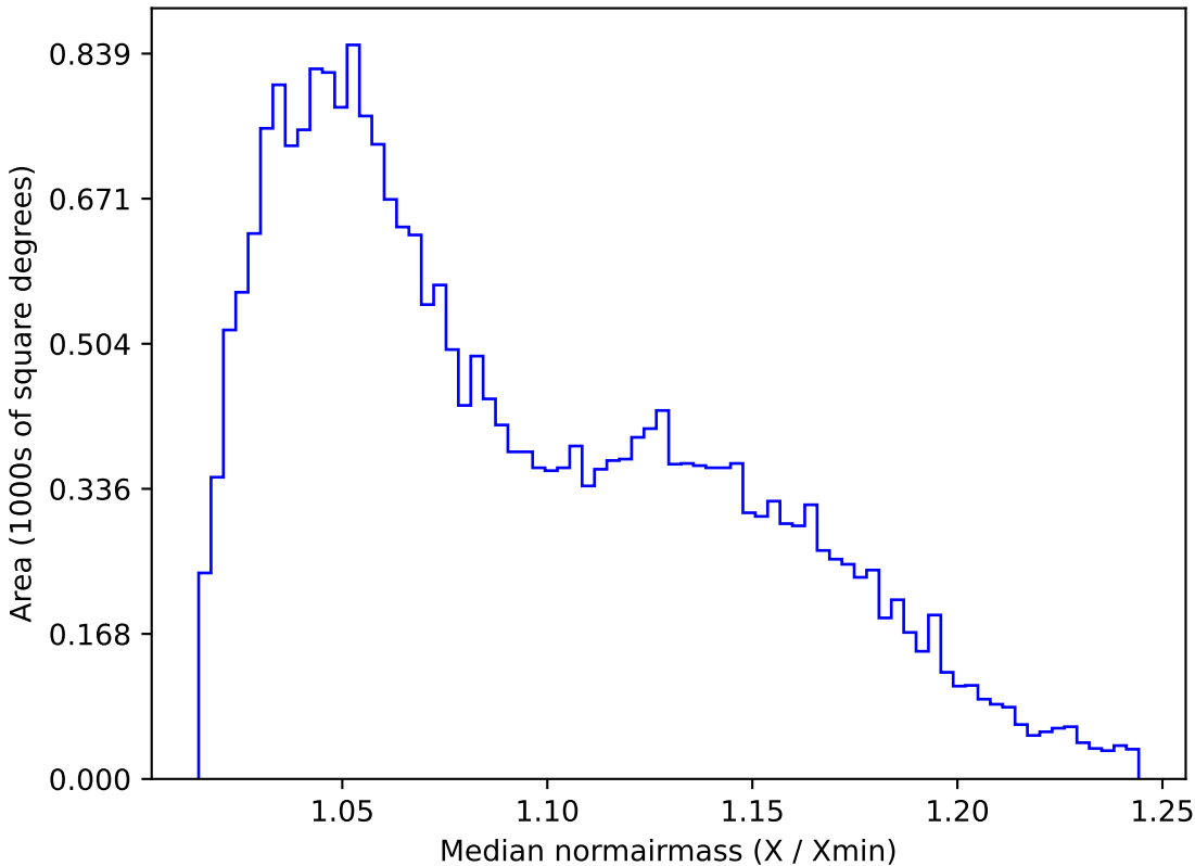
weather_cloudso10v3.4_10yrs All sky g band: Median normairmass
