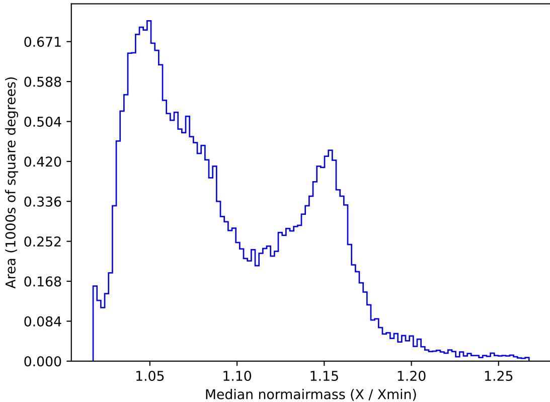
weather_cloudso10v3.4_10yrs All sky all bands: Median normairmass
