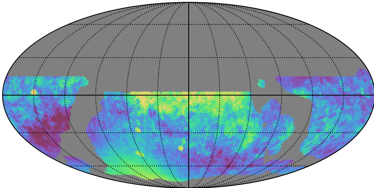
weather_cloudso10v3.4_10yrs WFD z band: Median moonDistance
