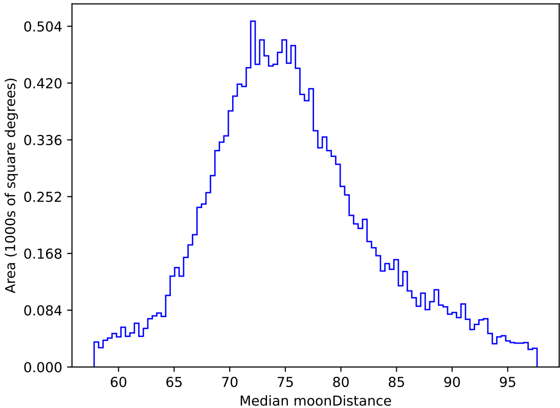
weather_cloudso10v3.4_10yrs WFD z band: Median moonDistance
