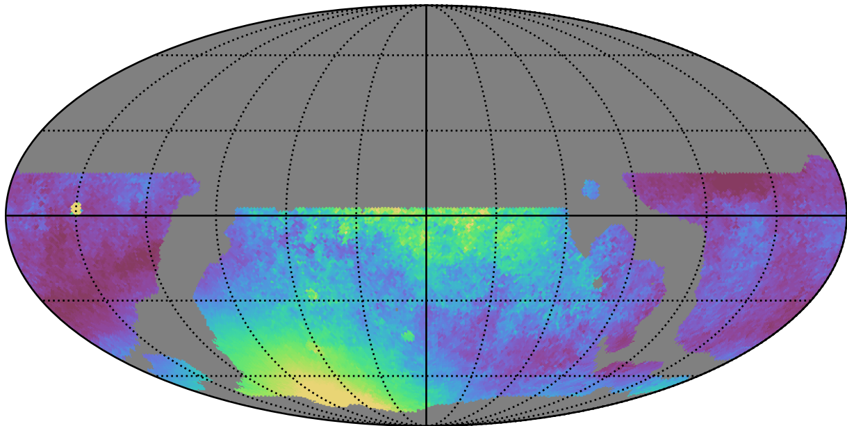
weather_cloudso10v3.4_10yrs WFD y band: Median moonDistance
