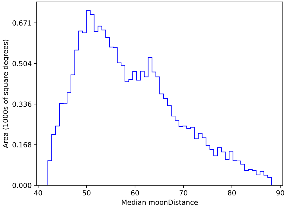
weather_cloudso10v3.4_10yrs WFD y band: Median moonDistance
