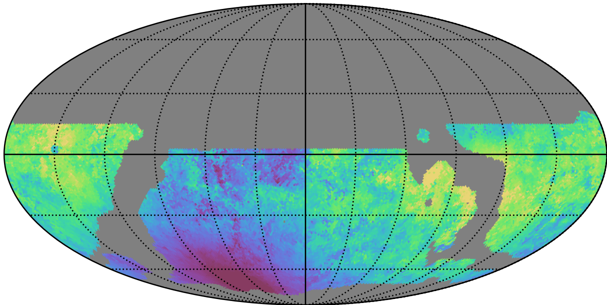
weather_cloudso10v3.4_10yrs WFD u band: Median moonDistance
