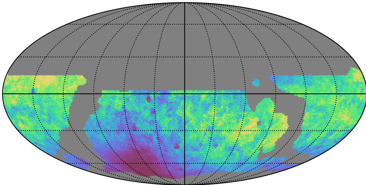
weather_cloudso10v3.4_10yrs WFD r band: Median moonDistance
