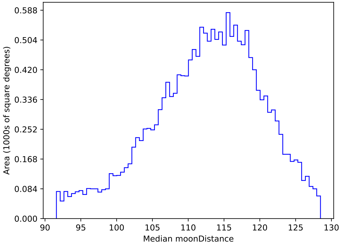
weather_cloudso10v3.4_10yrs WFD r band: Median moonDistance
