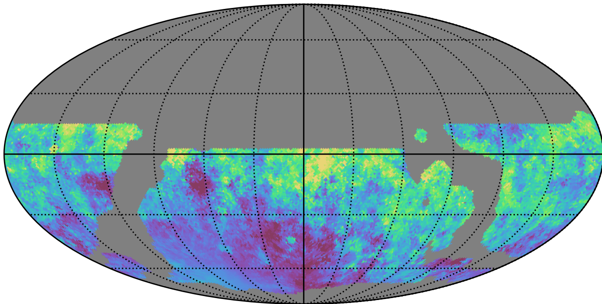
weather_cloudso10v3.4_10yrs WFD i band: Median moonDistance
