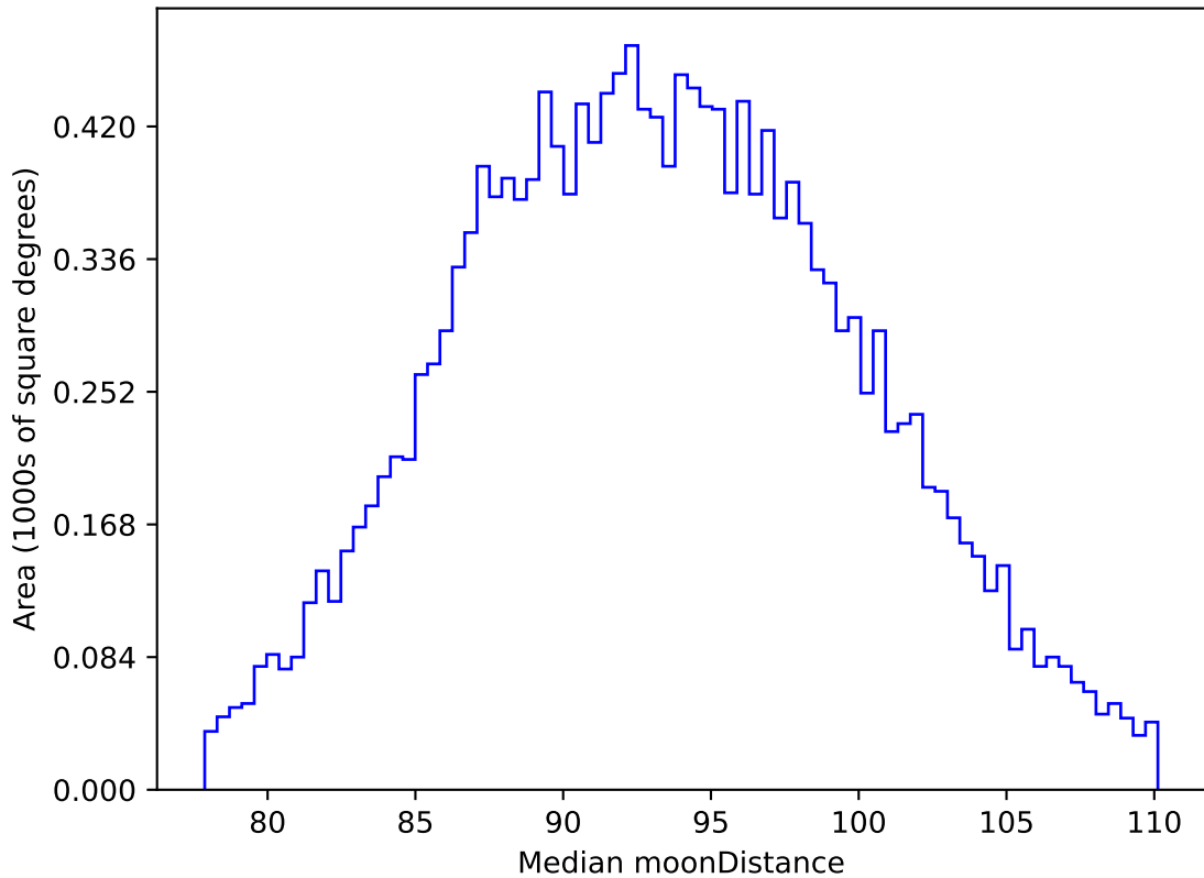
weather_cloudso10v3.4_10yrs WFD i band: Median moonDistance
