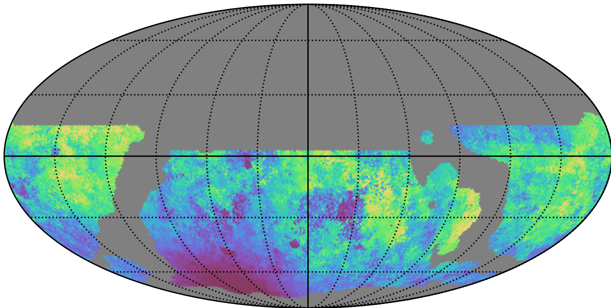
weather_cloudso10v3.4_10yrs WFD g band: Median moonDistance
