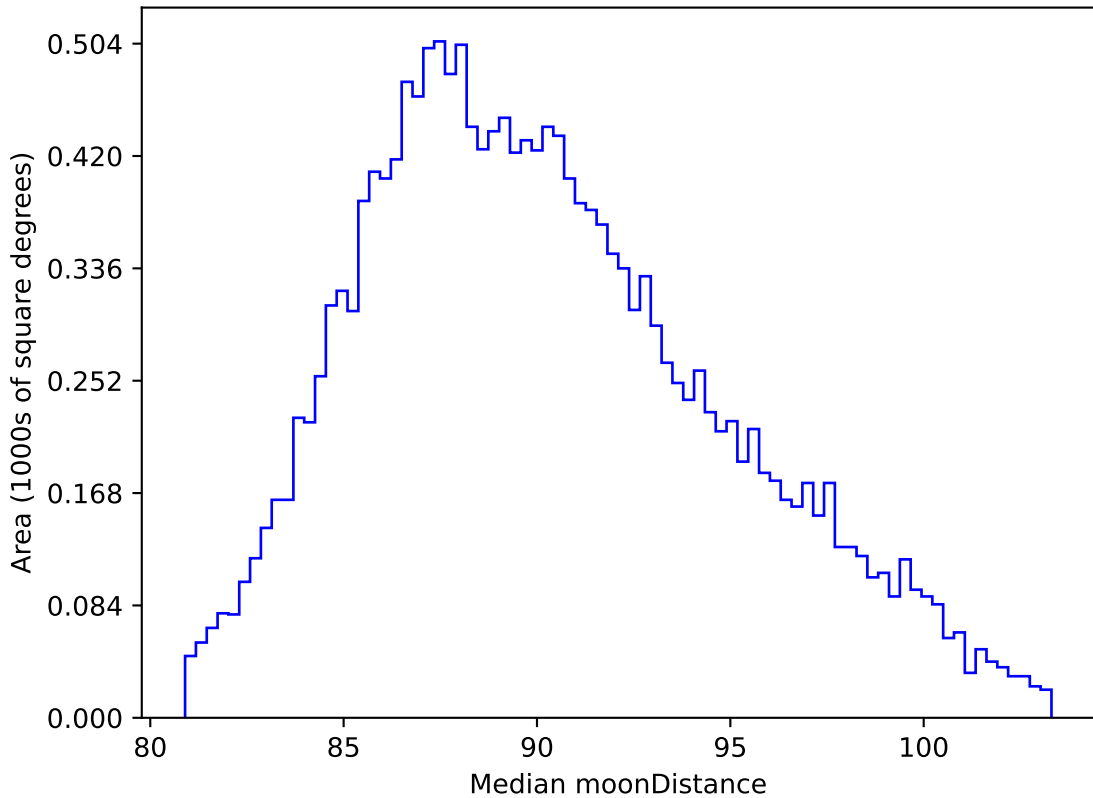
weather_cloudso10v3.4_10yrs WFD all bands: Median moonDistance
