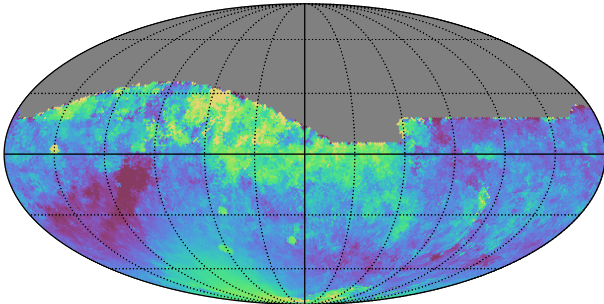
weather_cloudso10v3.4_10yrs All sky z band: Median moonDistance
