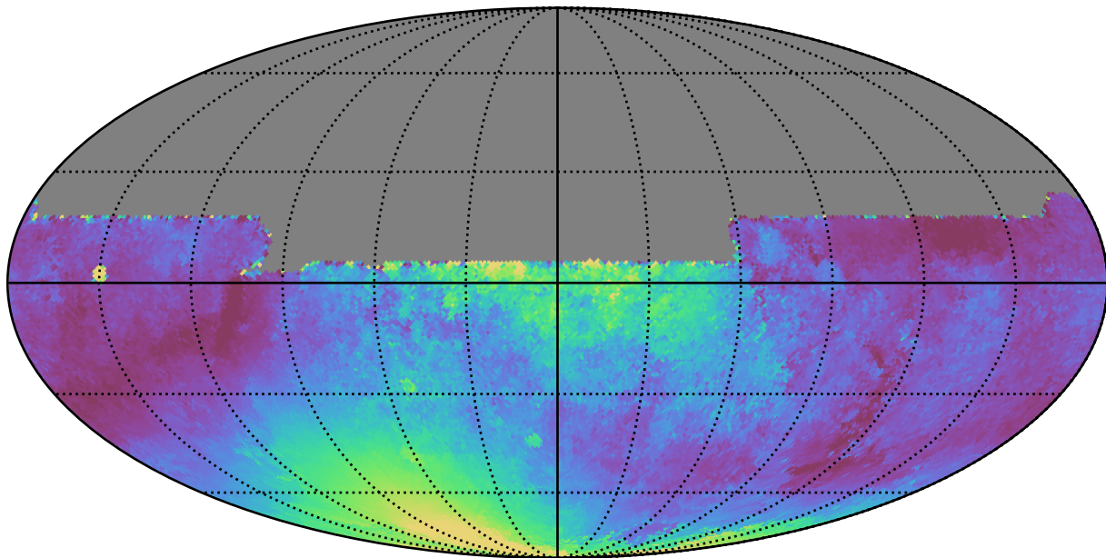
weather_cloudso10v3.4_10yrs All sky y band: Median moonDistance
