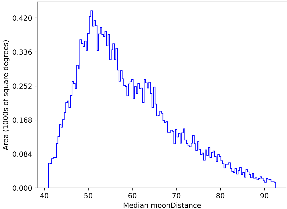
weather_cloudso10v3.4_10yrs All sky y band: Median moonDistance
