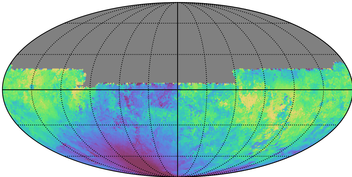
weather_cloudso10v3.4_10yrs All sky u band: Median moonDistance
