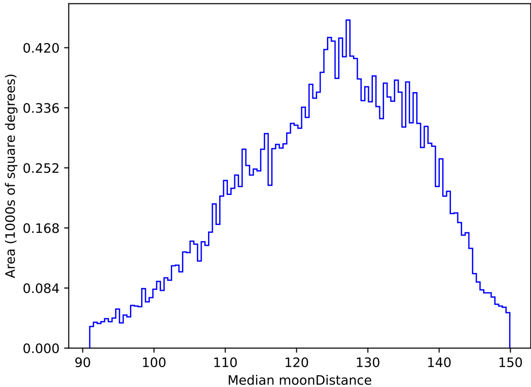
weather_cloudso10v3.4_10yrs All sky u band: Median moonDistance
