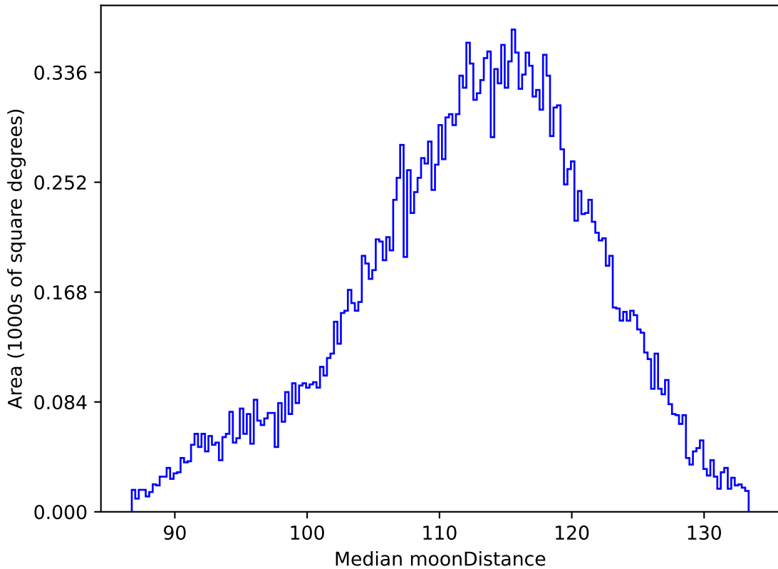
weather_cloudso10v3.4_10yrs All sky r band: Median moonDistance
