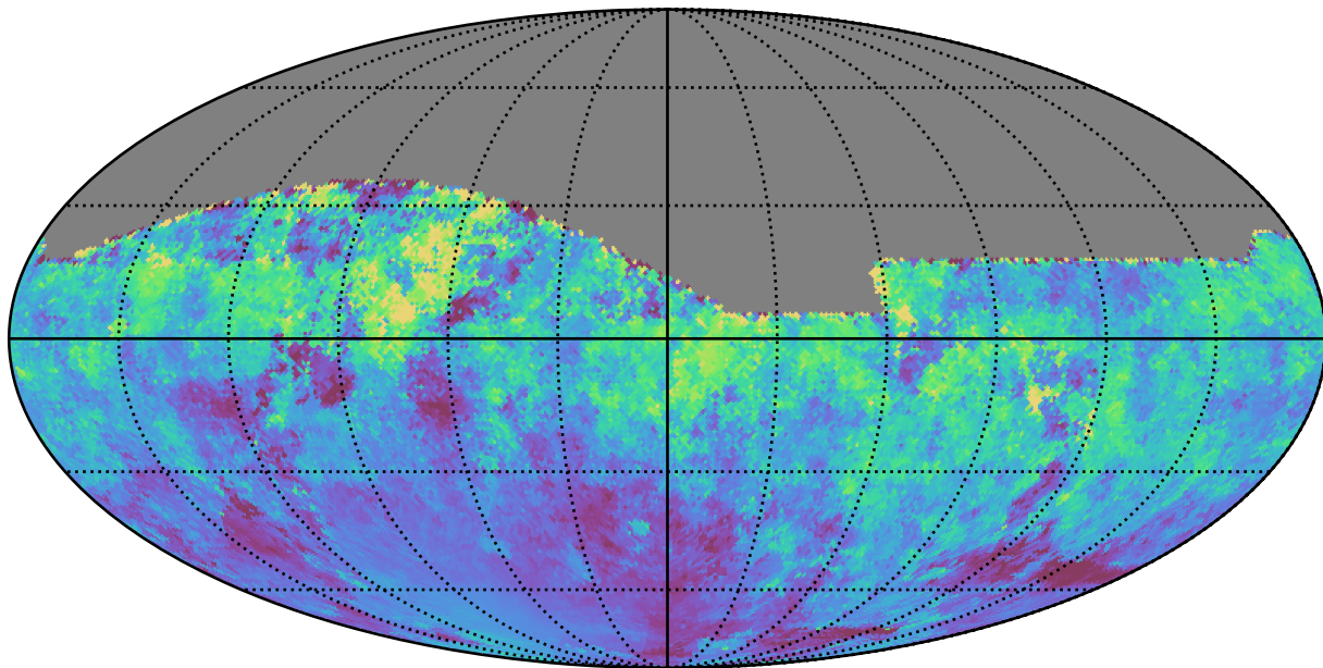
weather_cloudso10v3.4_10yrs All sky i band: Median moonDistance
