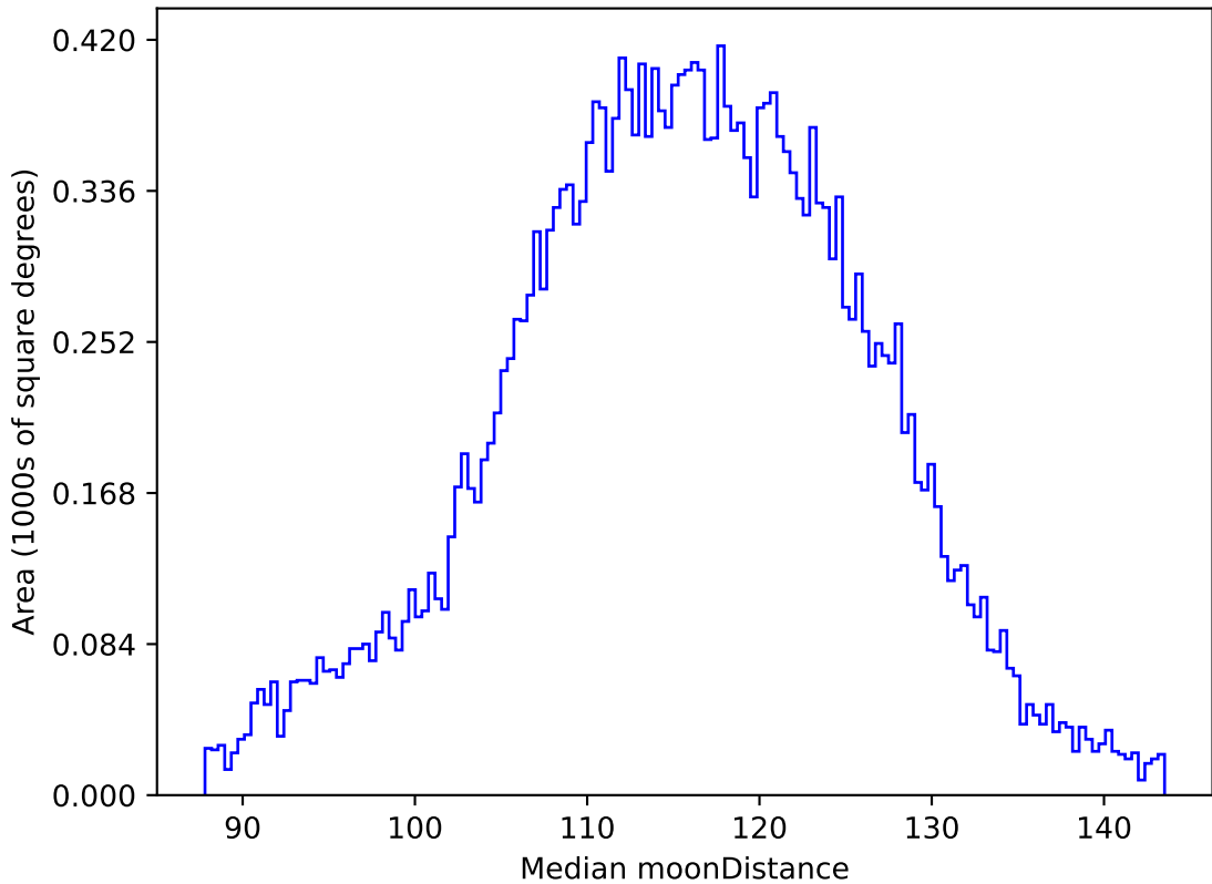
weather_cloudso10v3.4_10yrs All sky g band: Median moonDistance
