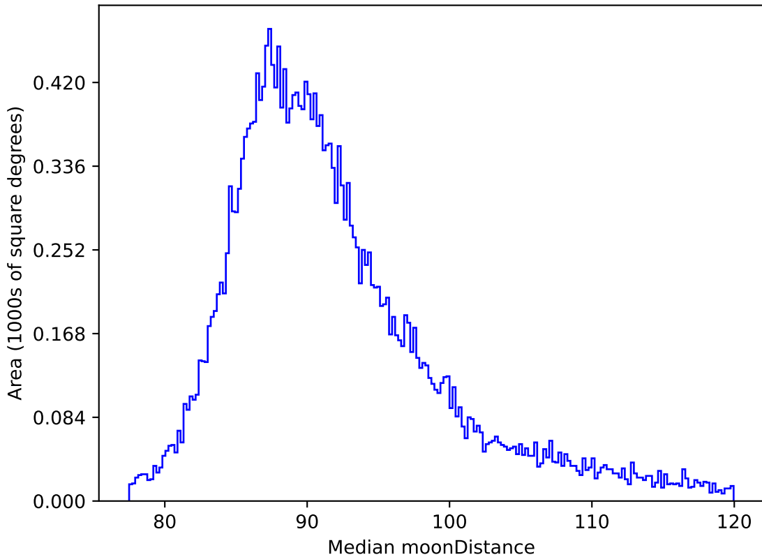
weather_cloudso10v3.4_10yrs All sky all bands: Median moonDistance
