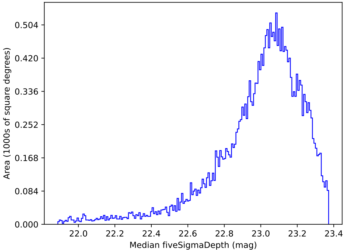
weather_cloudso10v3.4_10yrs Yr 1 z band: Median fiveSigmaDepth
