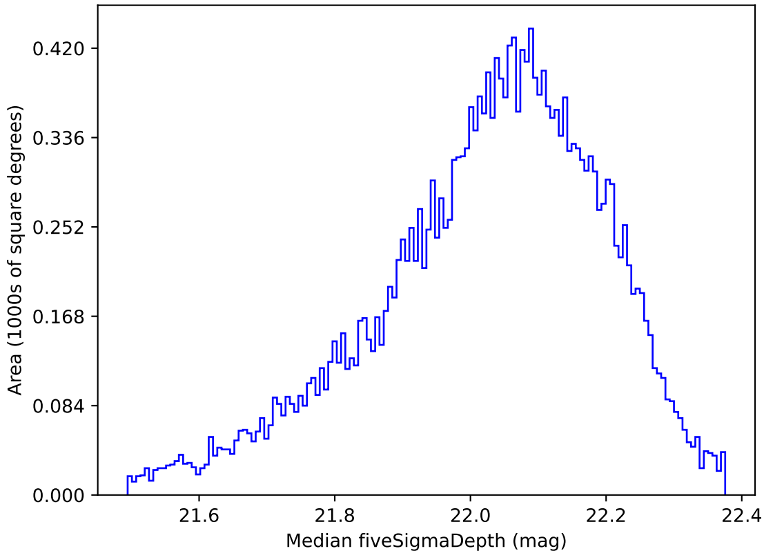
weather_cloudso10v3.4_10yrs Yr 1 y band: Median fiveSigmaDepth
