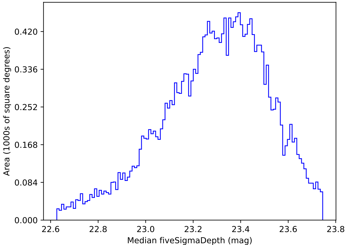
weather_cloudso10v3.4_10yrs Yr 1 u band: Median fiveSigmaDepth
