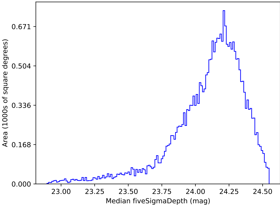
weather_cloudso10v3.4_10yrs Yr 1 r band: Median fiveSigmaDepth
