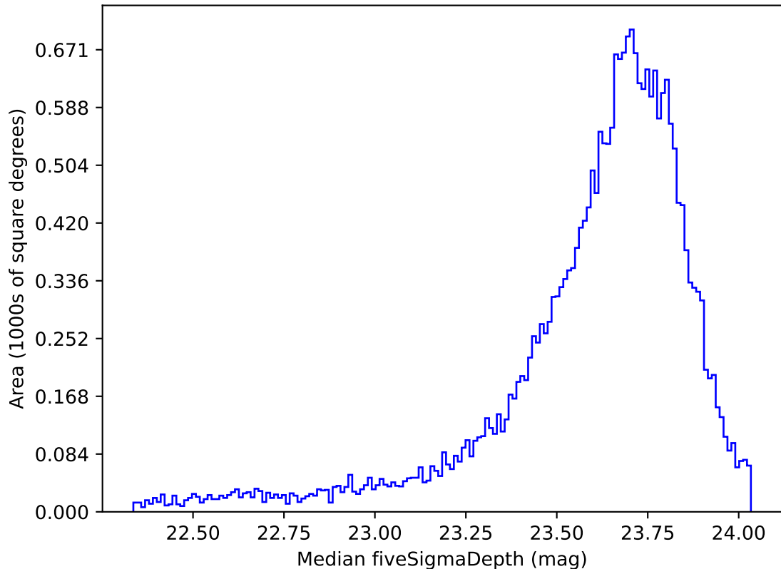
weather_cloudso10v3.4_10yrs Yr 1 i band: Median fiveSigmaDepth
