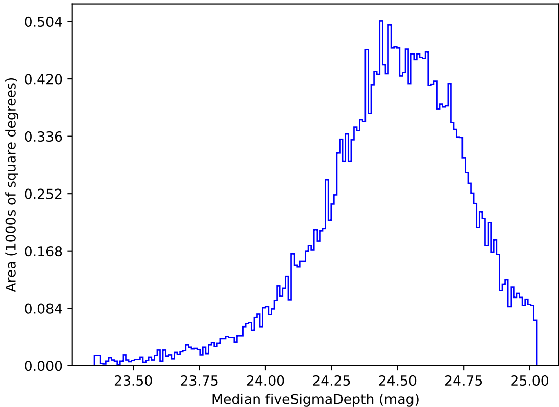
weather_cloudso10v3.4_10yrs Yr 1 g band: Median fiveSigmaDepth
