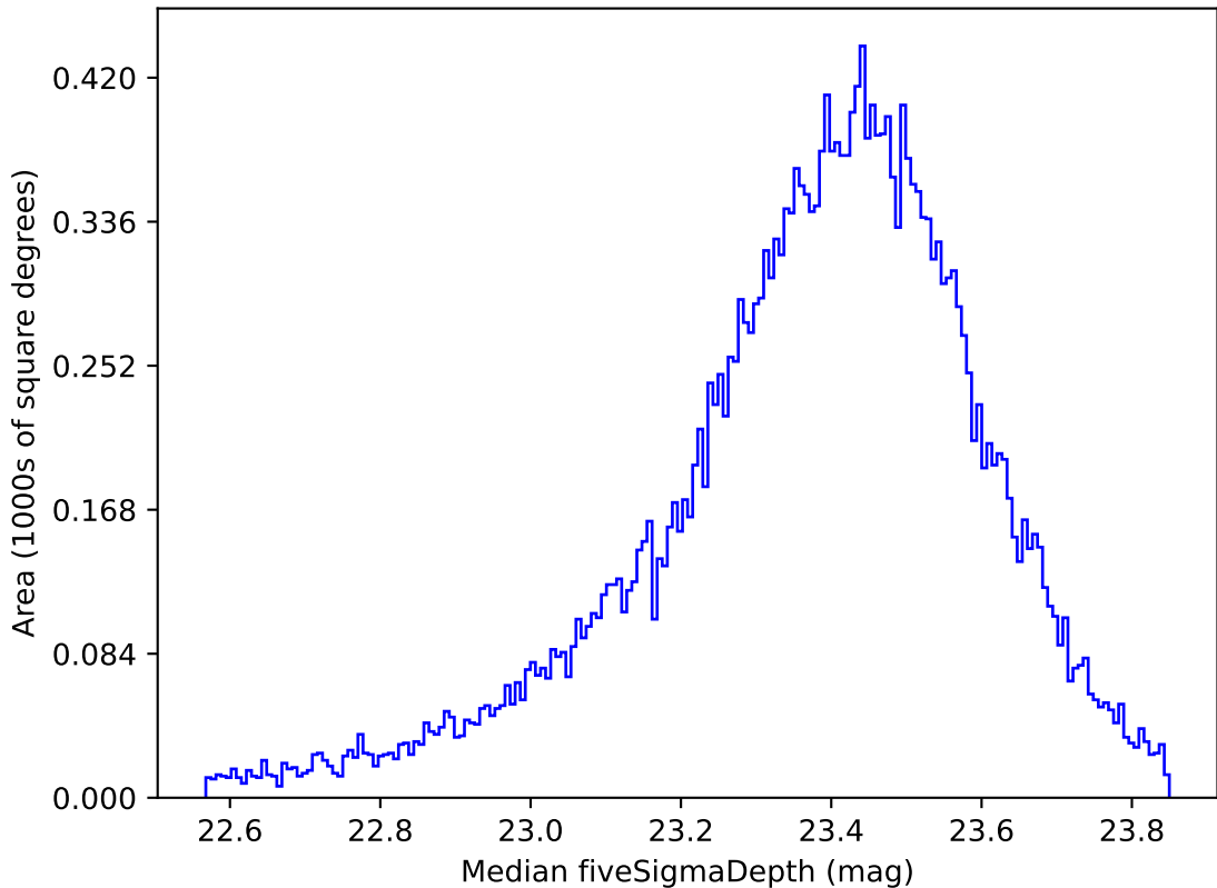
weather_cloudso10v3.4_10yrs Yr 1 all bands: Median fiveSigmaDepth
