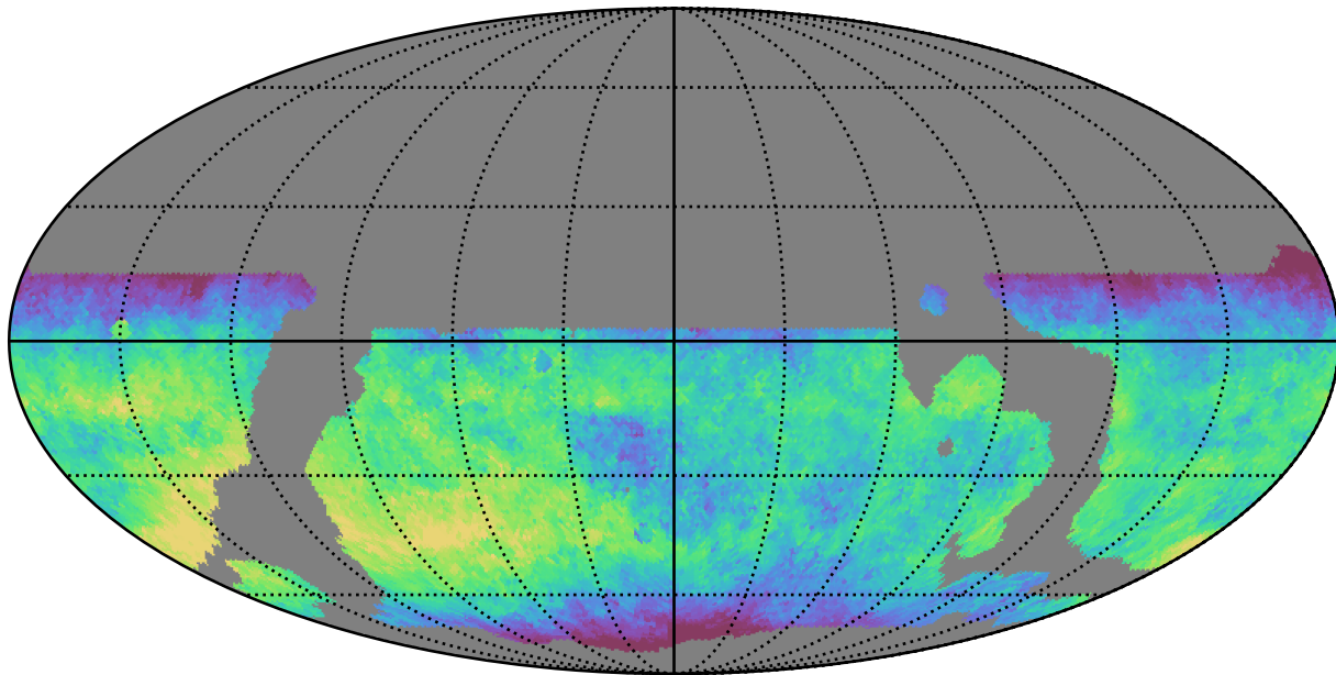
weather_cloudso10v3.4_10yrs WFD z band: Median fiveSigmaDepth
