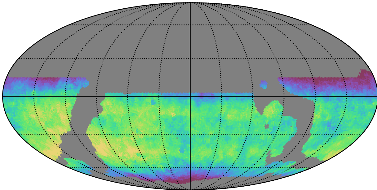
weather_cloudso10v3.4_10yrs WFD y band: Median fiveSigmaDepth
