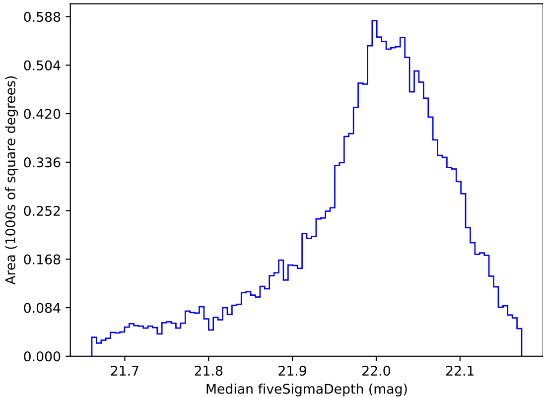
weather_cloudso10v3.4_10yrs WFD y band: Median fiveSigmaDepth
