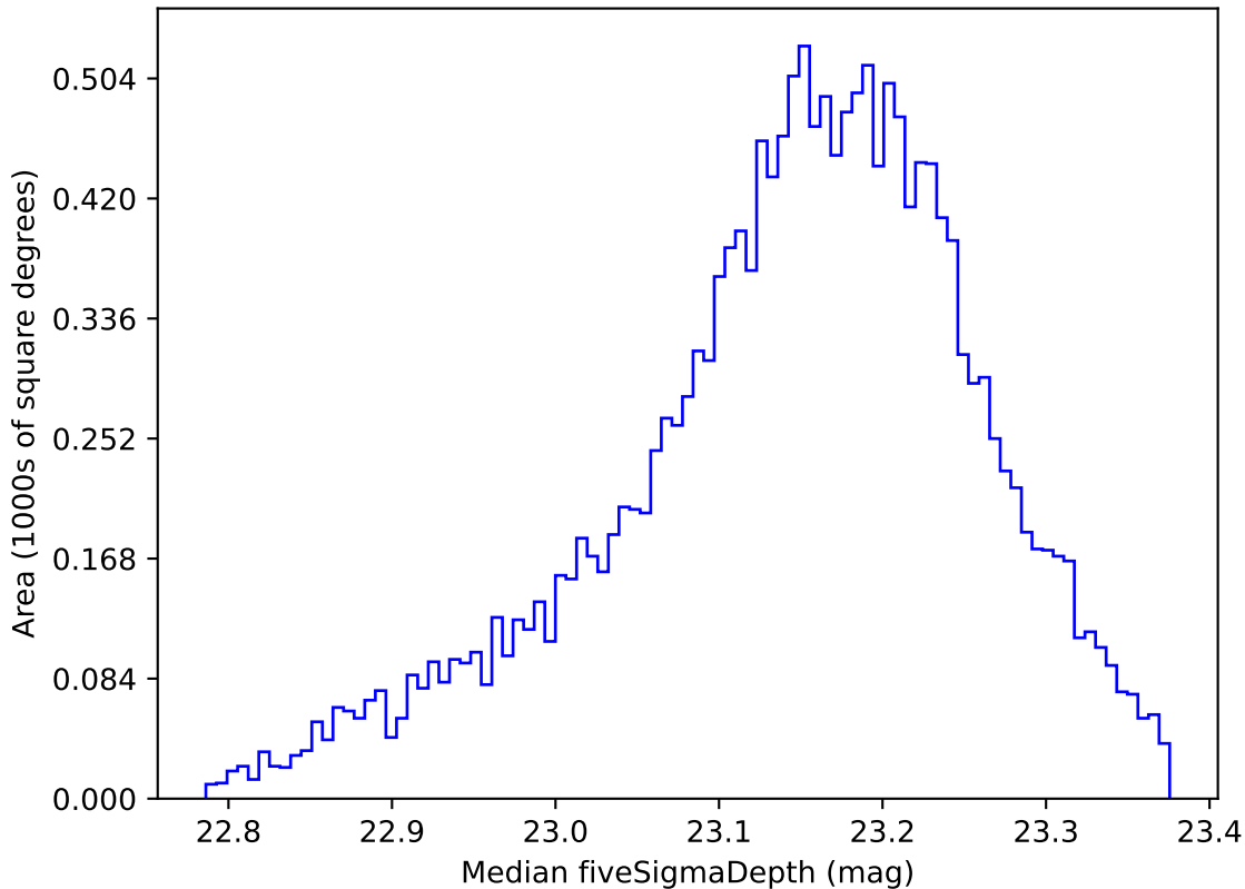
weather_cloudso10v3.4_10yrs WFD u band: Median fiveSigmaDepth
