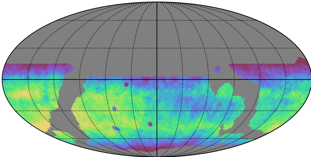
weather_cloudso10v3.4_10yrs WFD r band: Median fiveSigmaDepth
