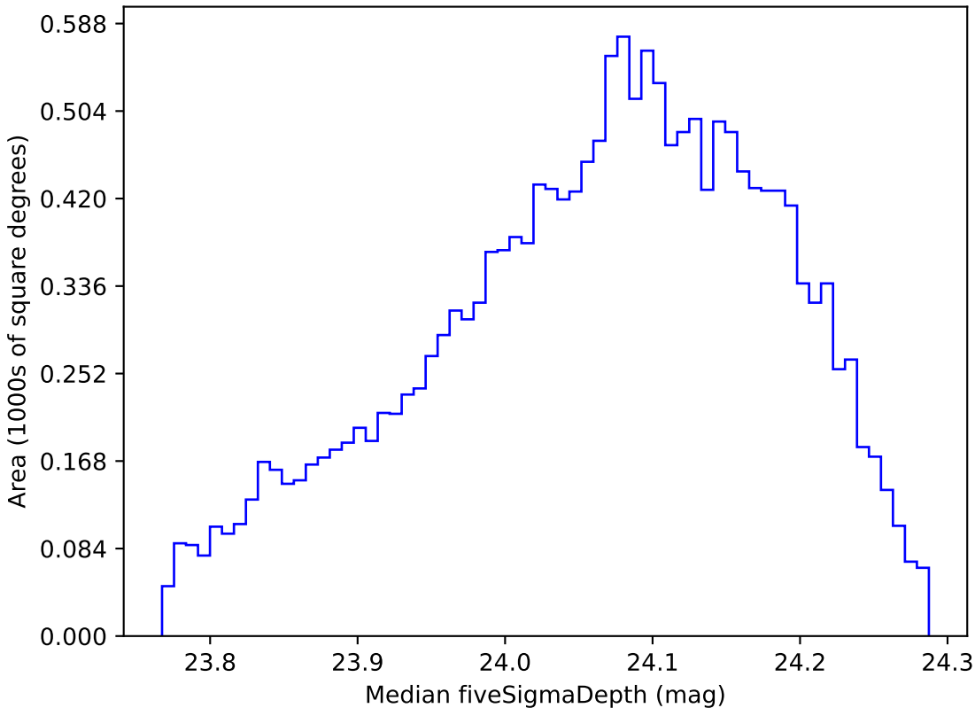
weather_cloudso10v3.4_10yrs WFD r band: Median fiveSigmaDepth
