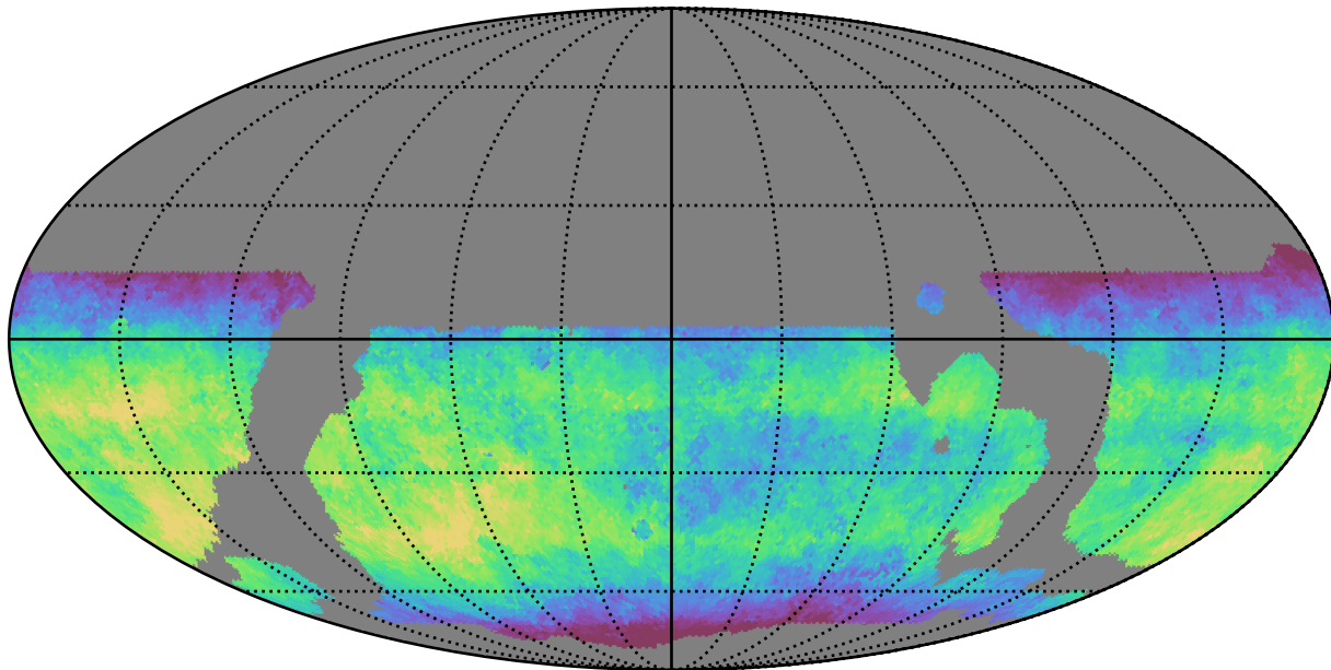
weather_cloudso10v3.4_10yrs WFD i band: Median fiveSigmaDepth
