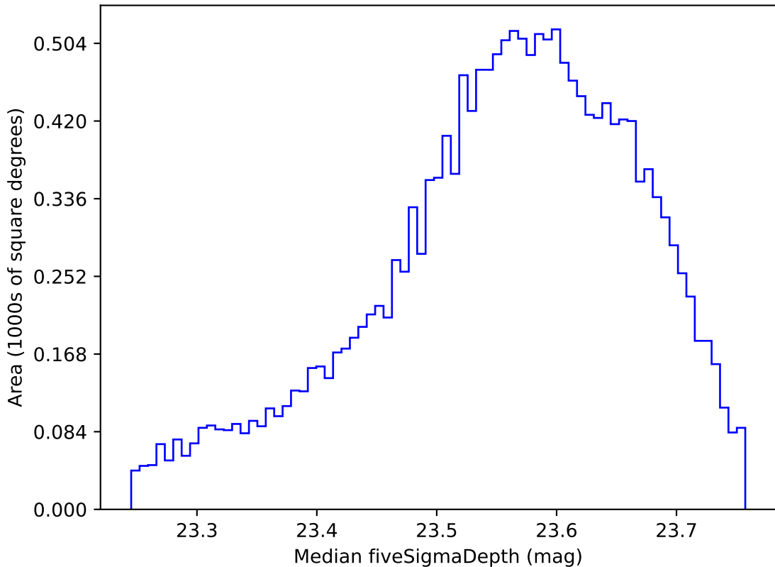
weather_cloudso10v3.4_10yrs WFD i band: Median fiveSigmaDepth
