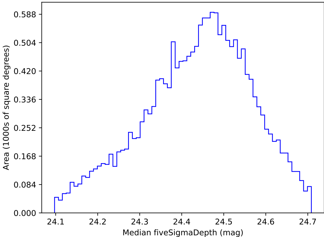
weather_cloudso10v3.4_10yrs WFD g band: Median fiveSigmaDepth
