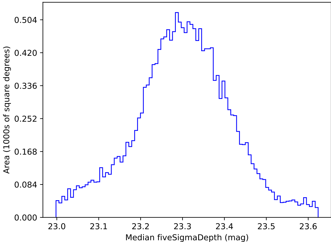
weather_cloudso10v3.4_10yrs WFD all bands: Median fiveSigmaDepth
