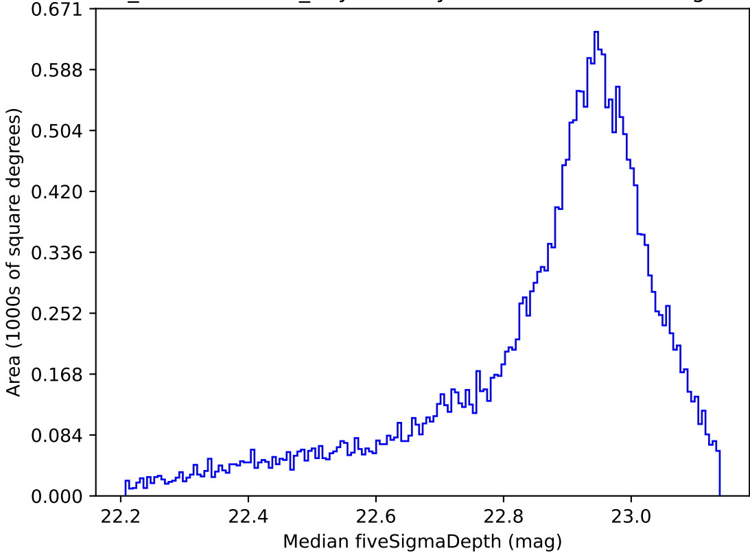
weather_cloudso10v3.4_10yrs All sky z band: Median fiveSigmaDepth
