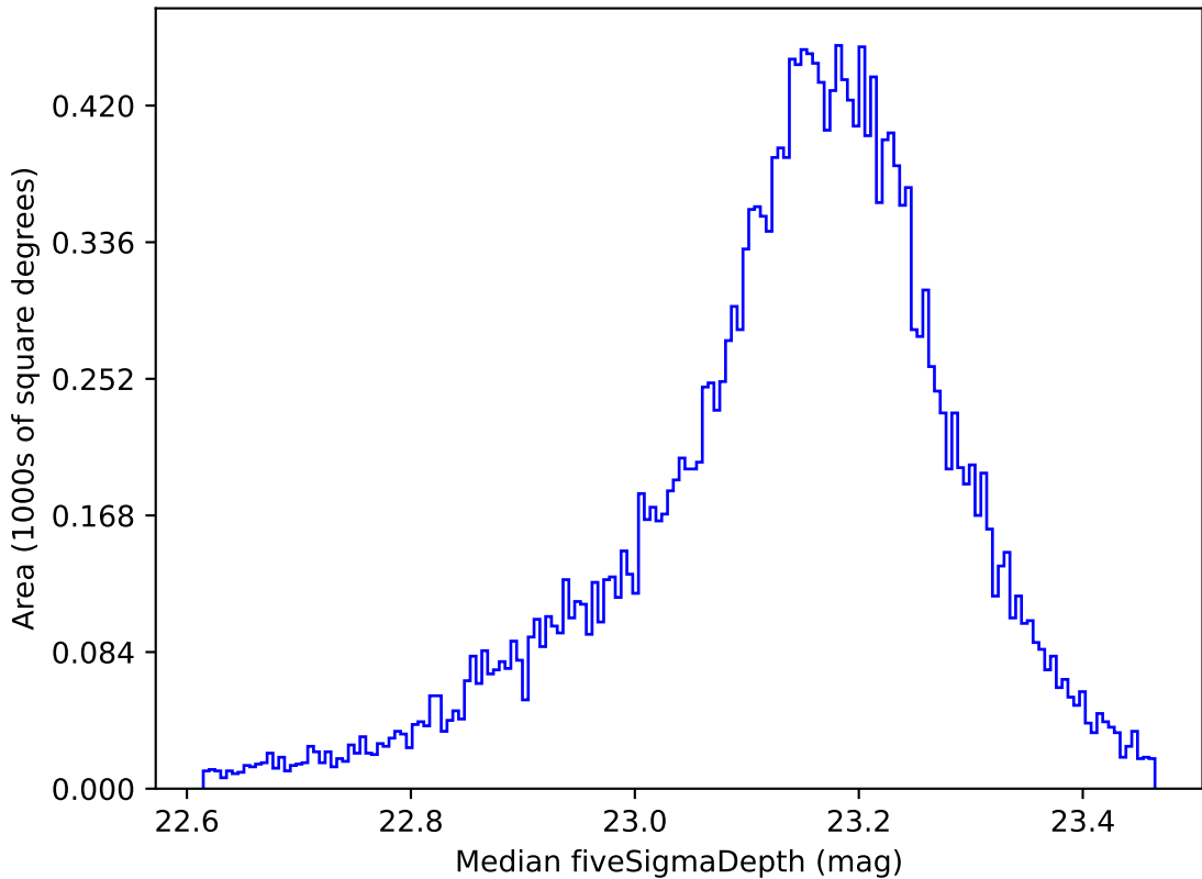
weather_cloudso10v3.4_10yrs All sky u band: Median fiveSigmaDepth
