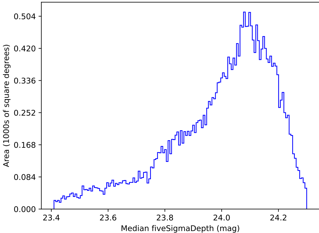
weather_cloudso10v3.4_10yrs All sky r band: Median fiveSigmaDepth
